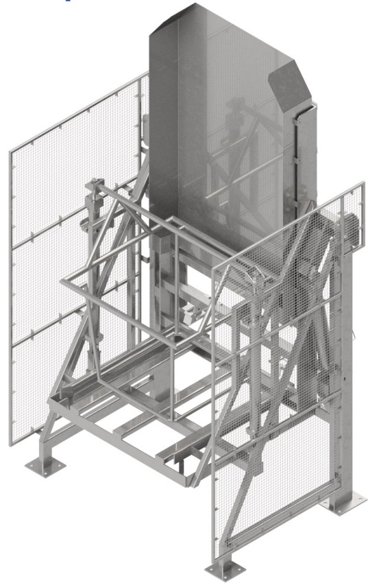
LE-BNB w/Bag-N-Box Hold-Down
