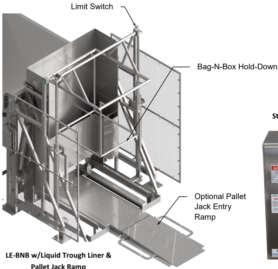
LE-BNB w/Bag-N-Box Hold-Down
