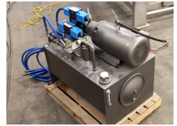
10 HP Hydraulic Power Unit w/Valves & Sloped Top Stainless Steel Cover
