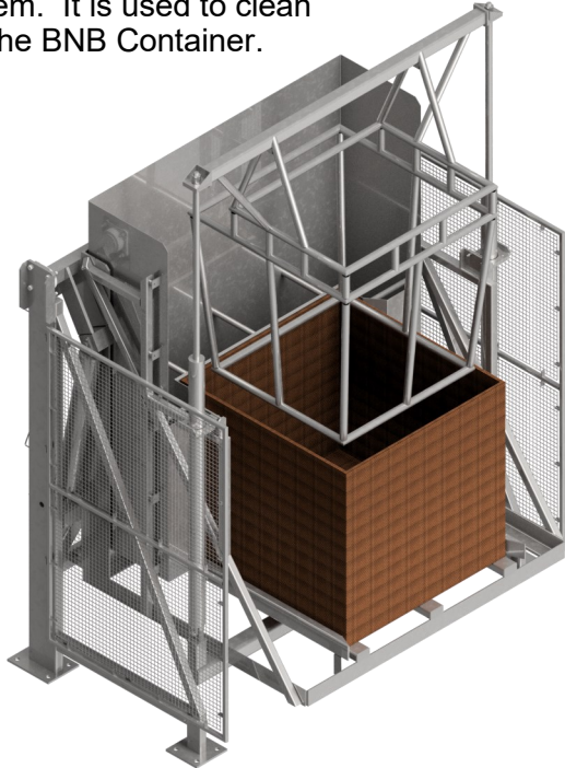
LE-BNB Carriage at Load-In, Hold-Down Raised
