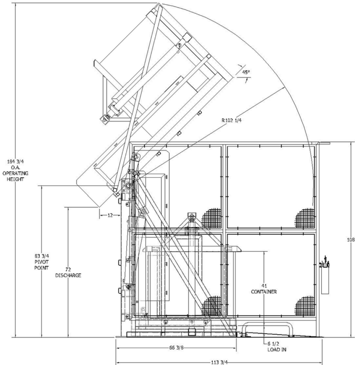
Typical LE-BNB Dumper Dimensions
