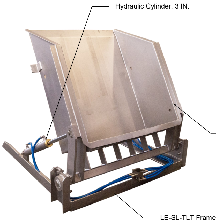
LE-SL-TLT Carriage Tilted 60 degrees
